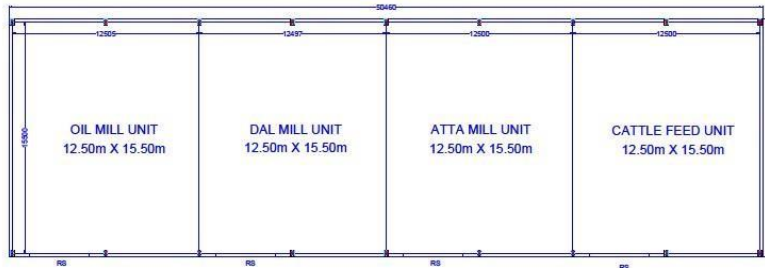
KEY PLAN OF GROUND FLOOR SCALE 1:200
