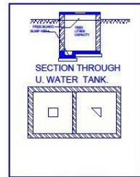
U.G WATER STORAGE TANK SCALE 1:200
